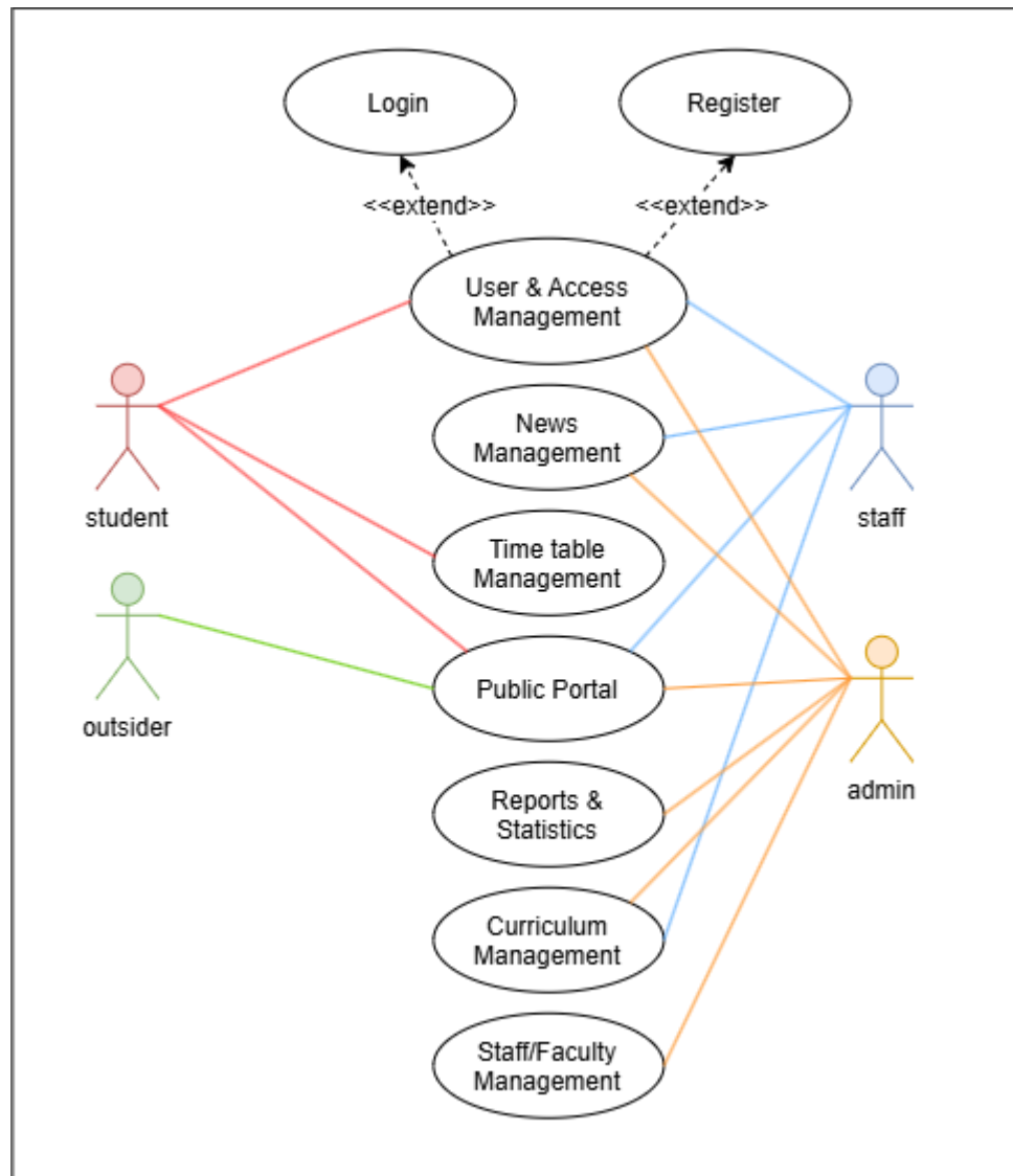
Use Case Diagram (UC-Main)
